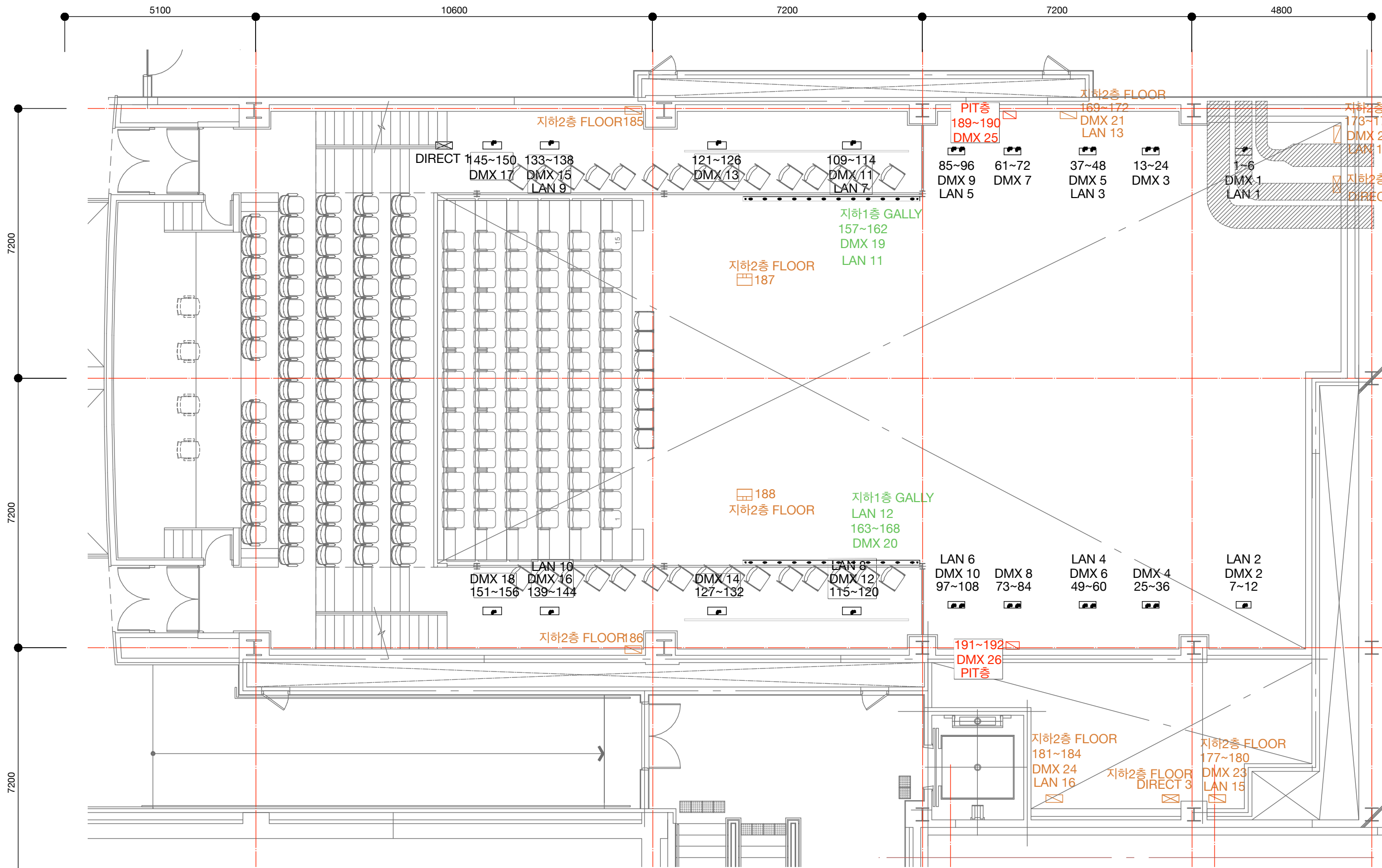
Sejong S Theatre Circuit Plan & DMX Adress
